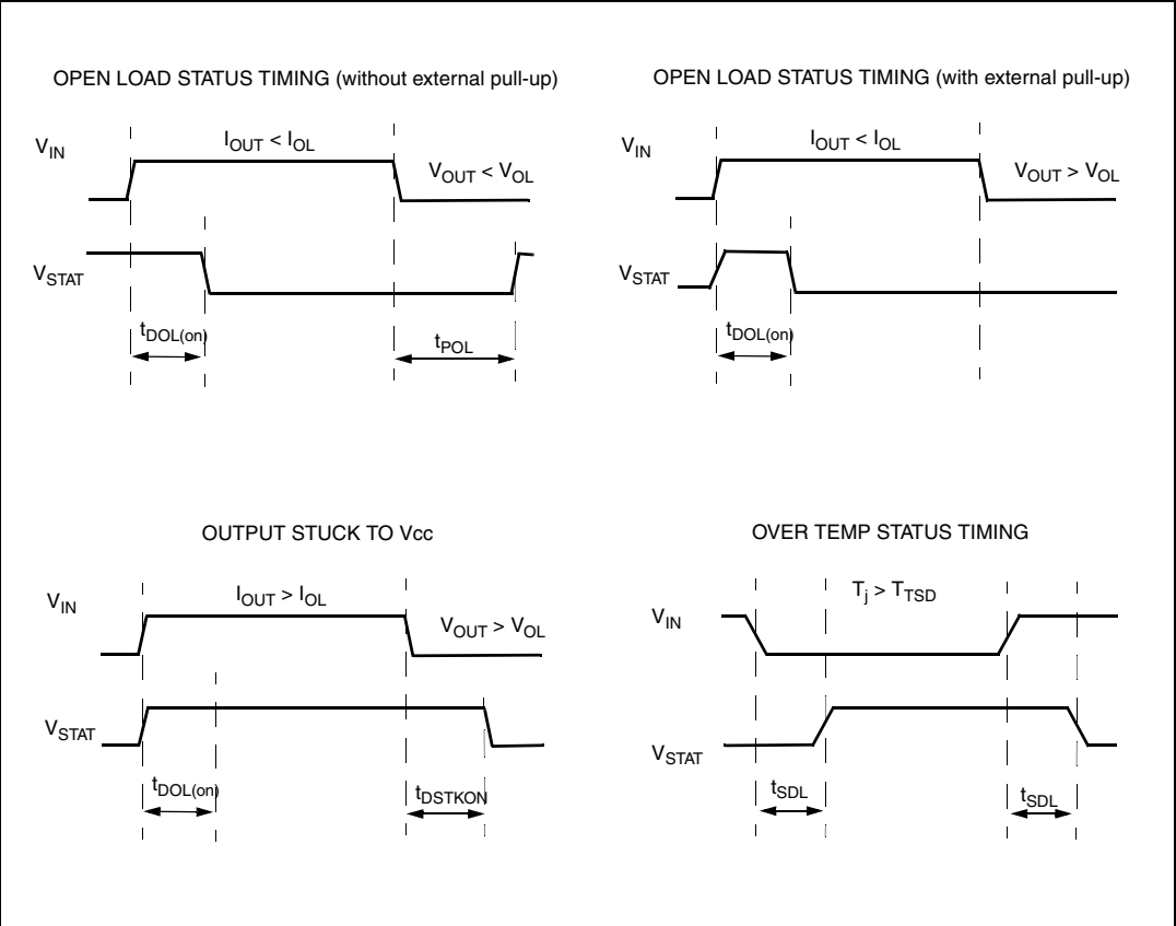
Figure 4. Status timings
