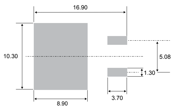
Figure 15. D 2 PAK recommended footprint (dimensions are in mm)
