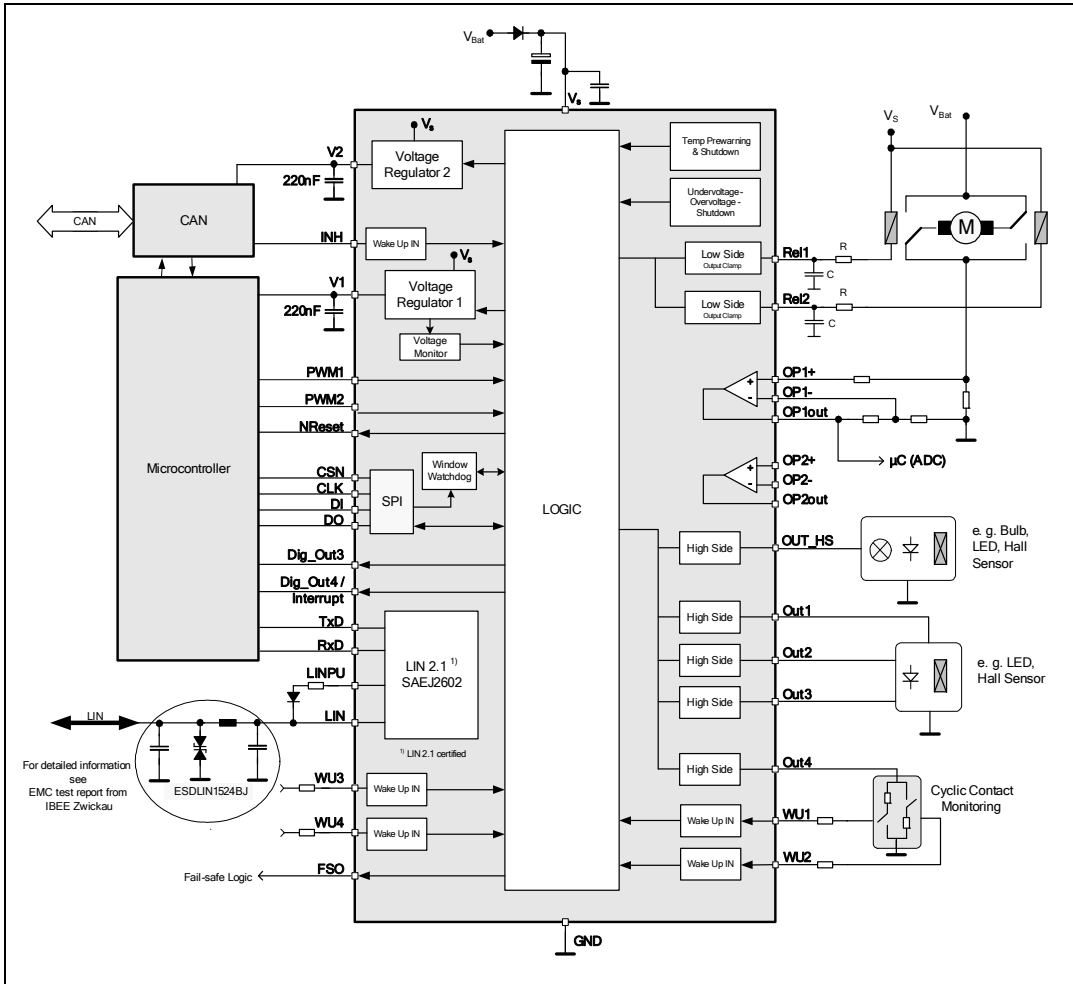
Figure 1. Block diagram
