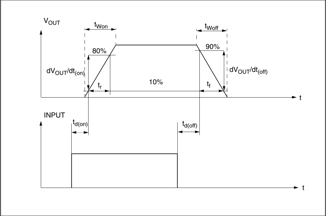
Figure 6. Switching characteristics
