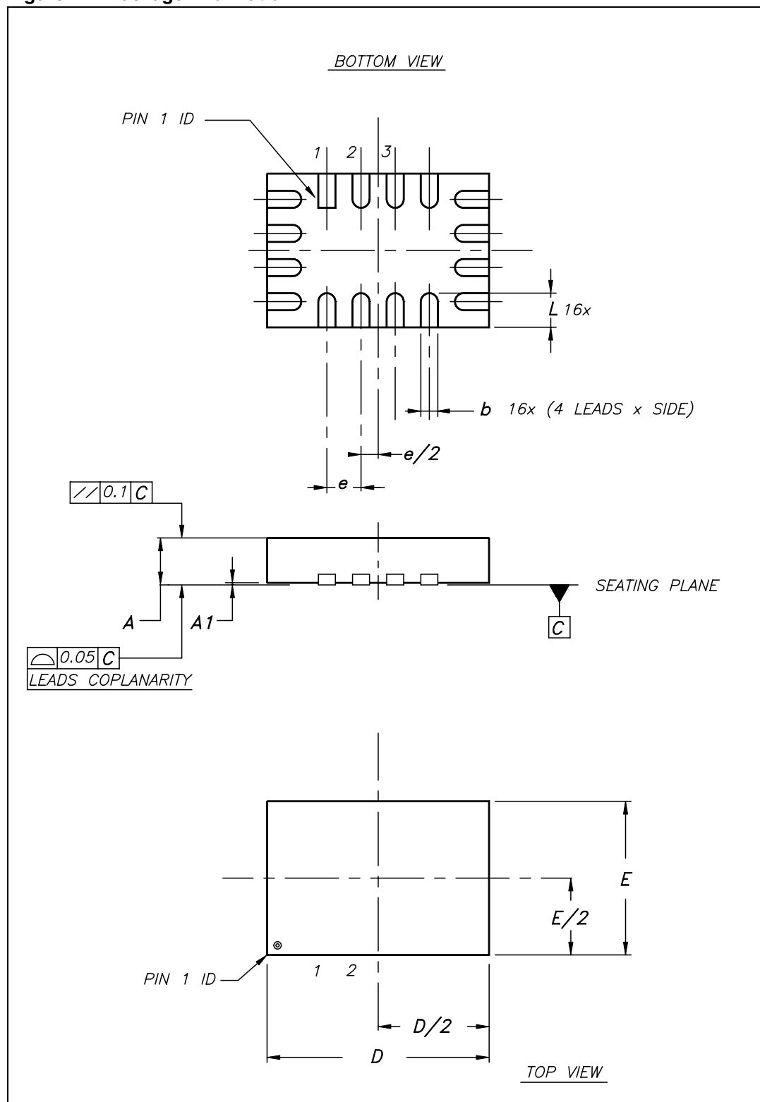
Figure 4. Package information
