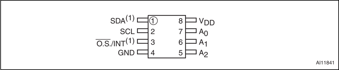
Figure 2. Connections
