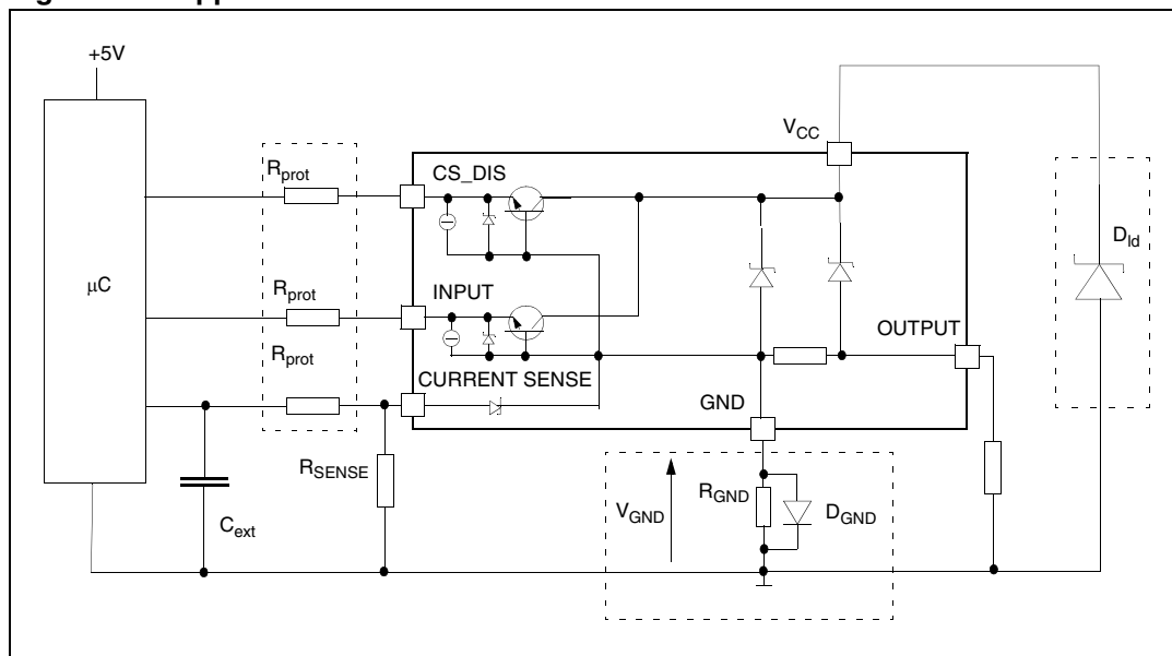
Figure 26. Application schematic
