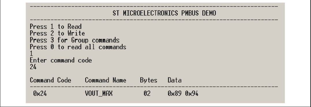
Figure 20. Read operation to check data writing
