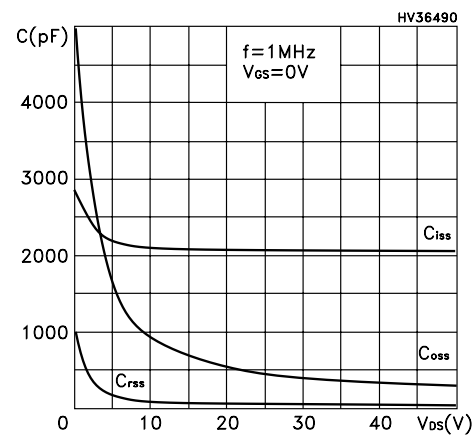
Figure 8. Capacitance variations
