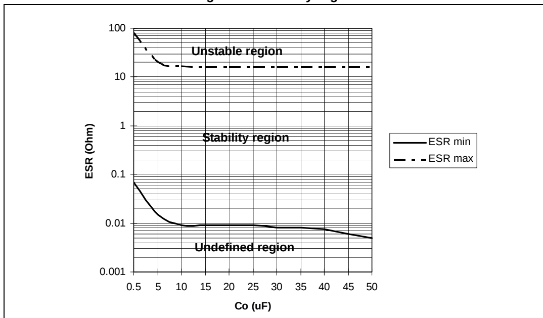
Figure 27. Stability region
