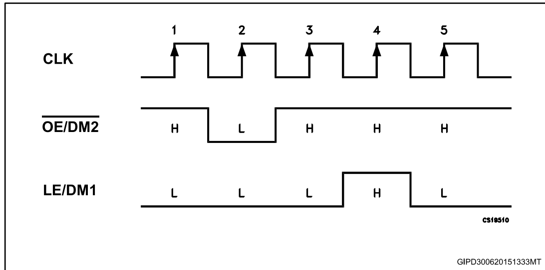
Figure 15: Entering in detection timing diagram
