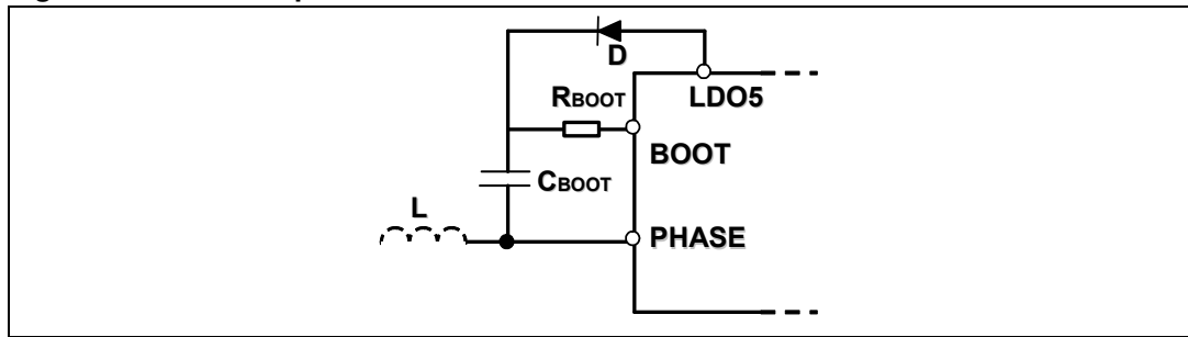
Figure 40. Bootstrap circuit
