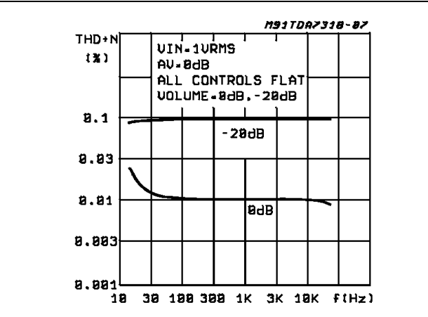
Figure 9. Distortion and noise vs. frequency (V IN = 1 V)
