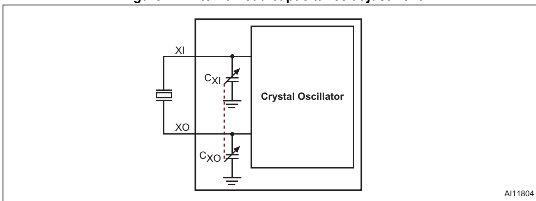
Figure 17. Internal load capacitance adjustment
