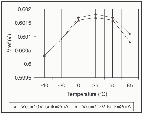
Figure 3. V_{ref} vs. temperature
