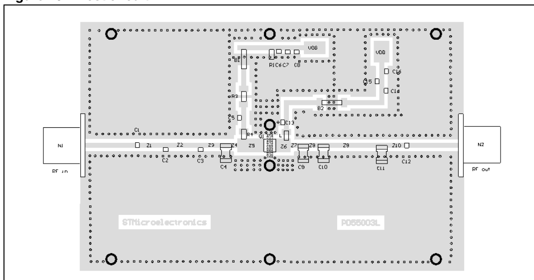
Figure 16. Test circuit
