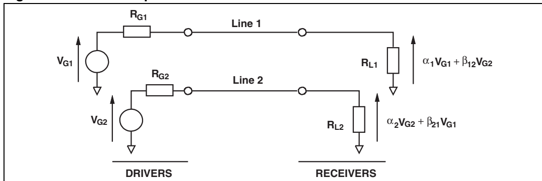
Figure 15. Crosstalk phenomena
