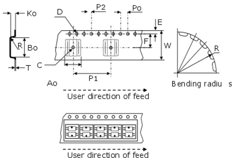
Figure 20. Tape specifications
