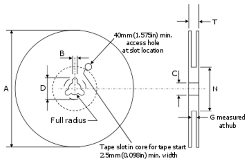
Figure 21. Reel specifications
