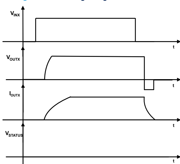
Figure 8. Switching on light inductive load
