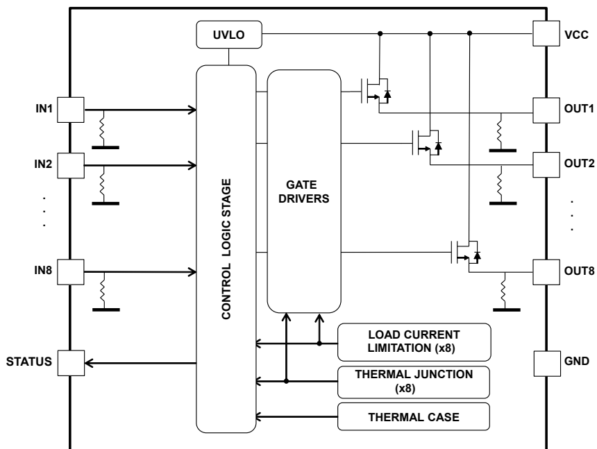
Figure 1. Internal schematic
