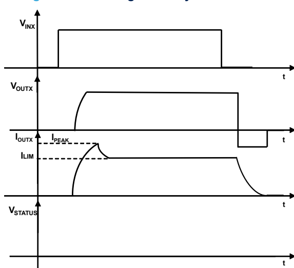
Figure 9. Switching on heavy inductive load
