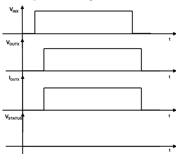
Figure 6. Switching on resistive load
