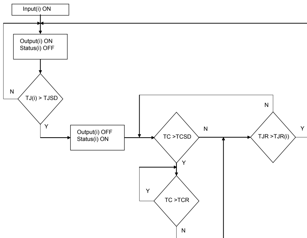
Figure 12. Thermal protection logic
