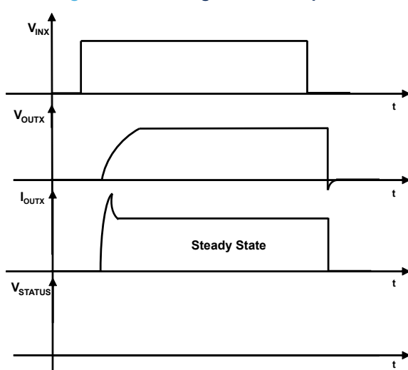
Figure 7. Switching on bulb lamp load
