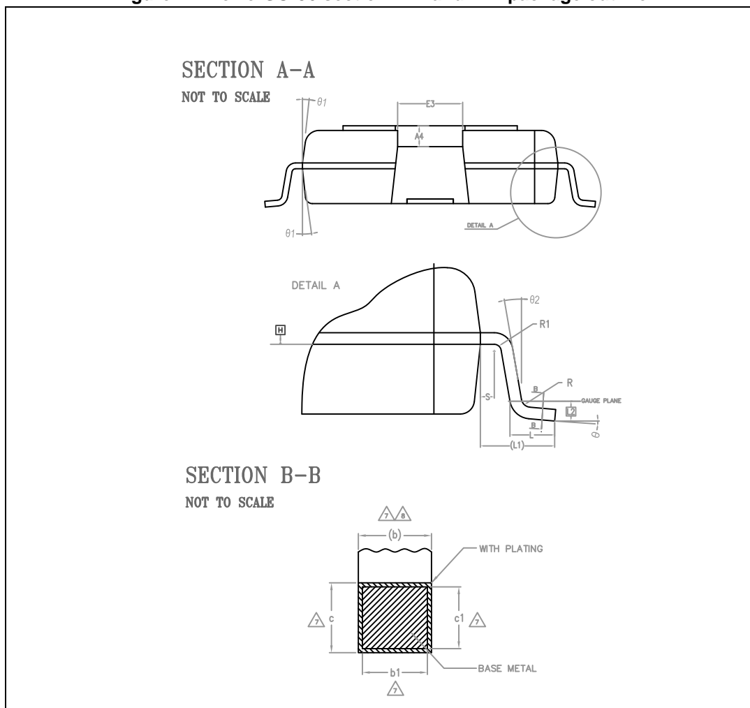
Figure 12. PowerSO-36 section A-A and B-B package outline
