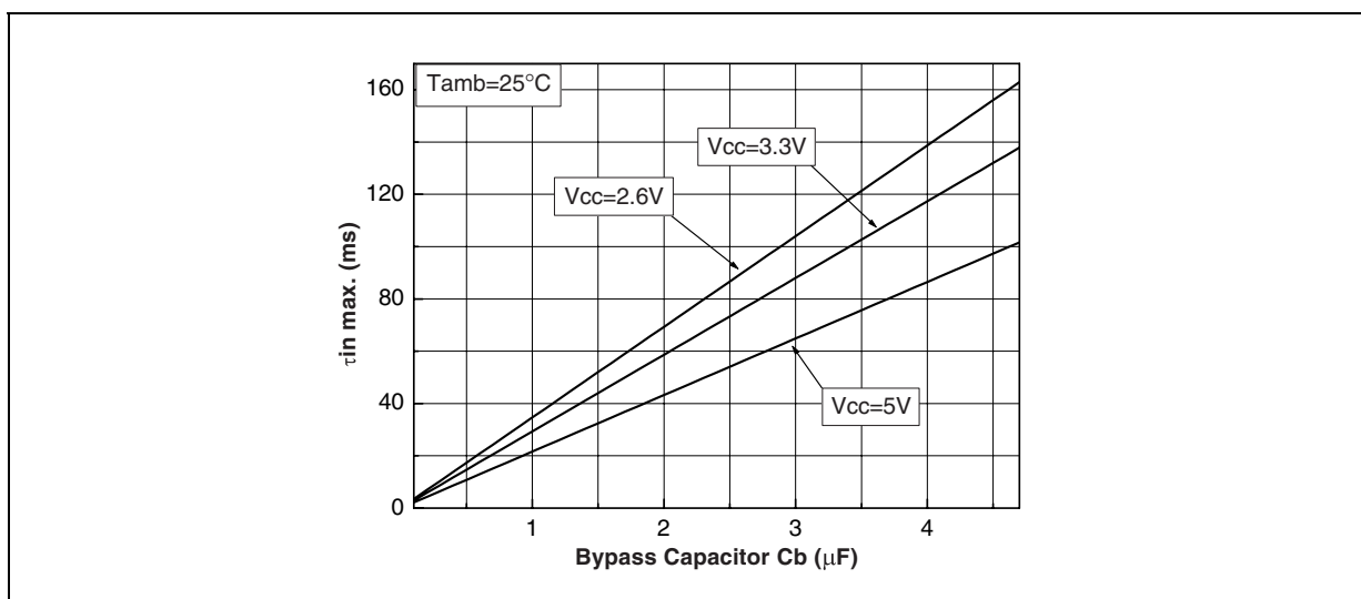
Figure 68: \tau_{in} max. versus bypass capacitor
