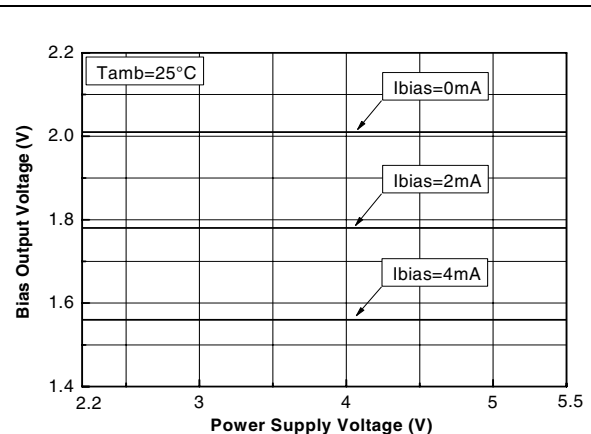
Figure 9. Bias output voltage vs. power supply voltage
