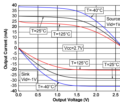
Figure 12. Output current vs. output voltage at V_{CC}=2.7\text{ V}
