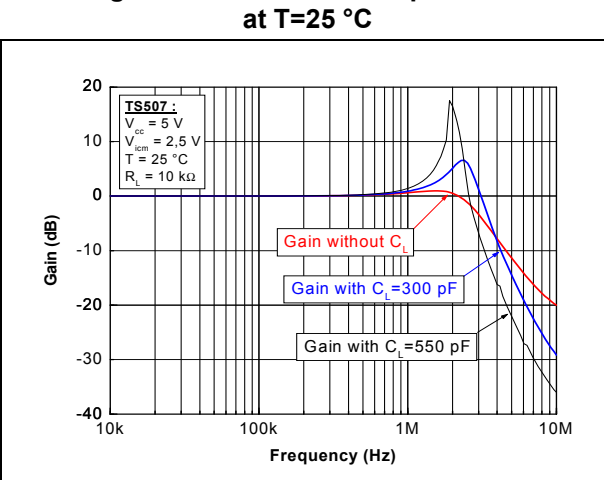
Figure 18. Closed loop gain in voltage follower configuration for different capacitive load at T=25^\circ\text{C}
