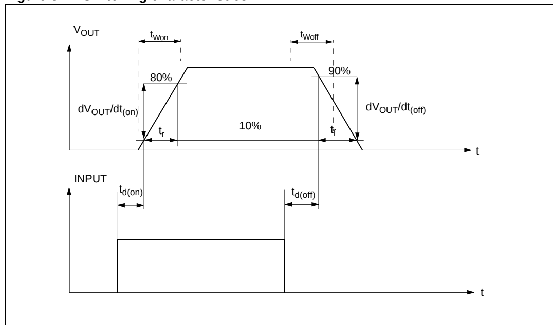
Figure 6. Switching characteristics
