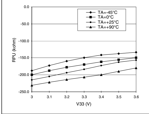
Figure 17. R_{PU} vs. V_{33} with V_{IN}=V_{SS}
