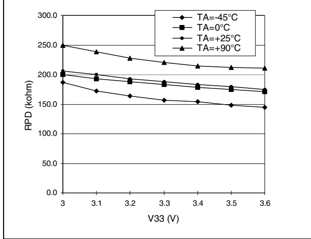
Figure 19. R_{PD} vs. V_{33} with V_{IN}=V_{33}
