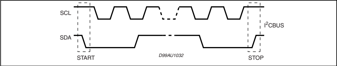
Figure 26. Timing diagram on the I 2 C bus
