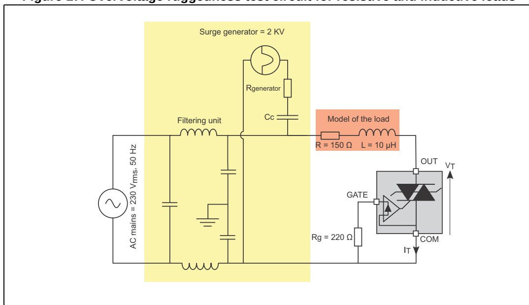
Figure 17. Overvoltage ruggedness test circuit for resistive and inductive loads
