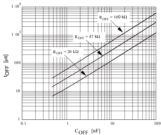
Figure 11. t_{OFF} versus C_{OFF} and R_{OFF}
