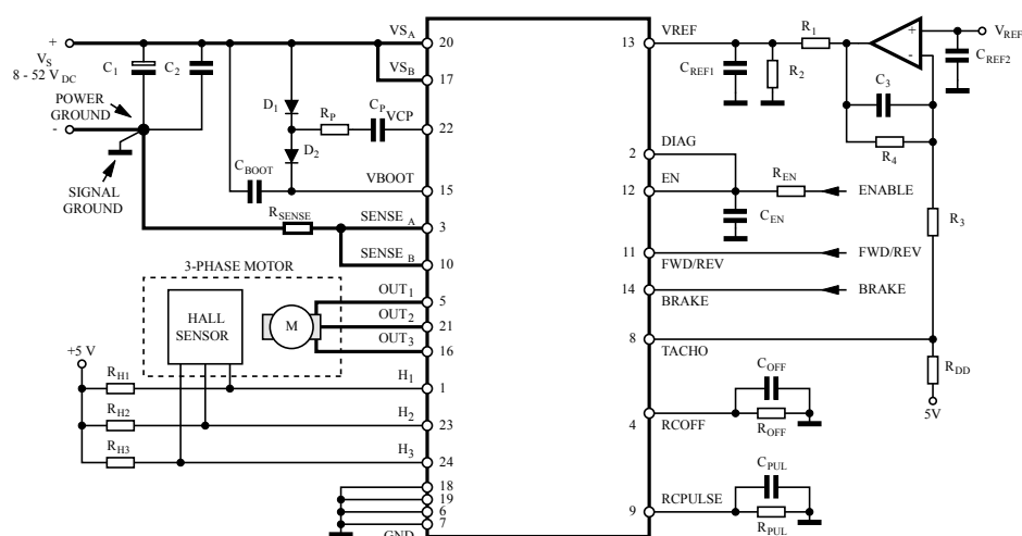
Figure 23. Typical application
