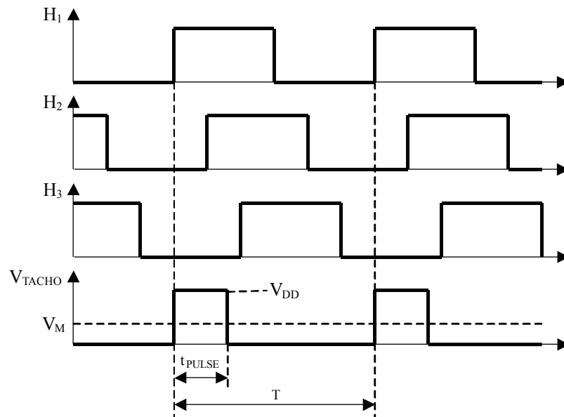
Figure 16. TACHO operation waveforms
