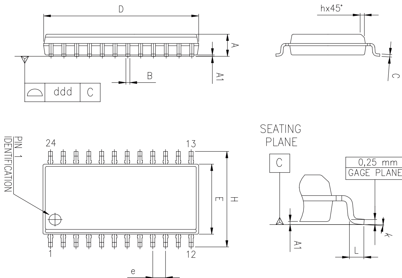
Figure 29. SO24 package outline
