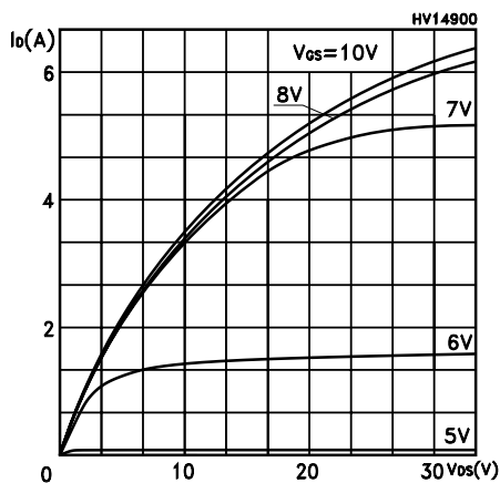
Figure 3. Output characteristics
