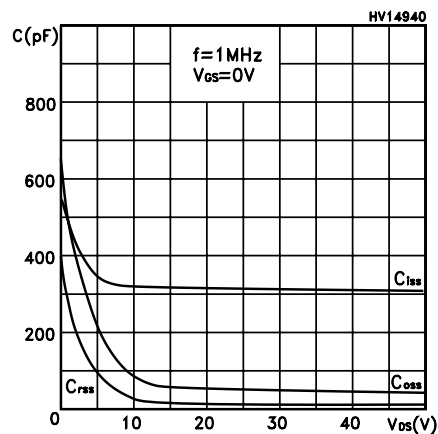
Figure 5. Capacitance variations
