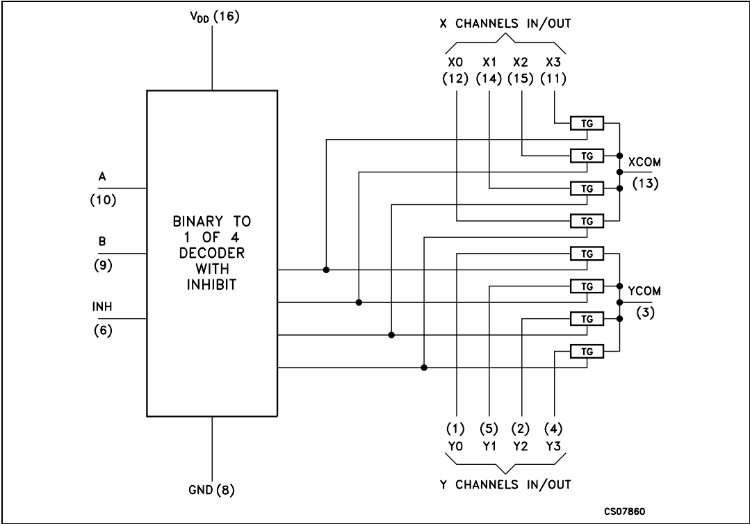
Figure 4. Functional diagram
