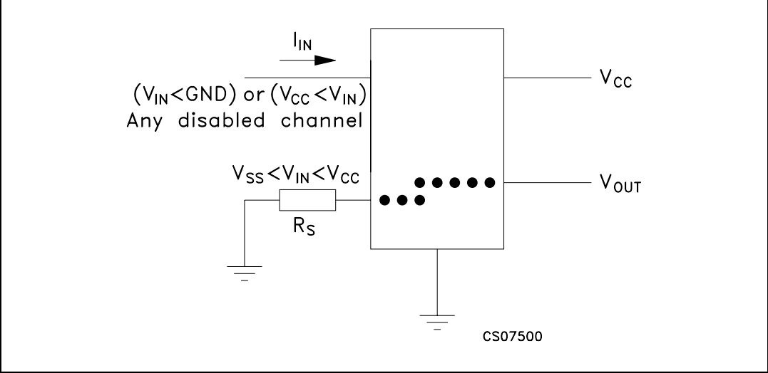
Figure 6. Test circuit 2
