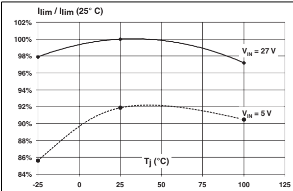
Figure 5. Typical current limiter variation versus junction temperature 0.9\text{ V} < V_{\text{OUT}} < 2\text{ V}
