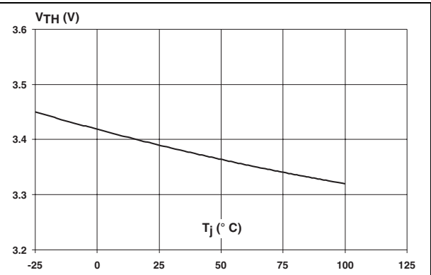
Figure 6. Typical limiter threshold voltage variation versus junction temperature for I_{\text{IN}} = 2.1\text{ mA}
