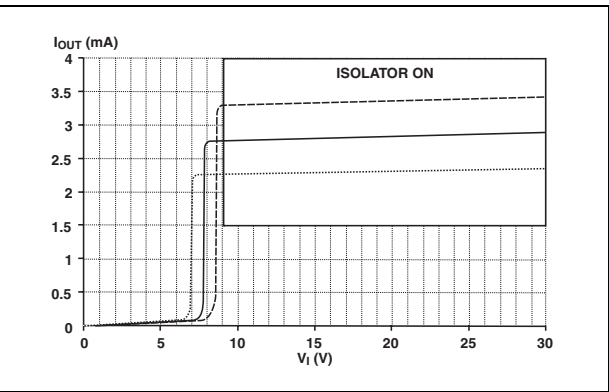
Figure 8. Transconductance characteristic
