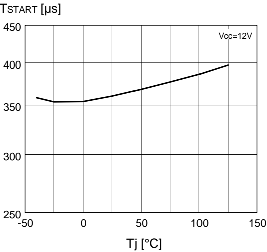
Figure 11. Start-up timer period vs. TJ
