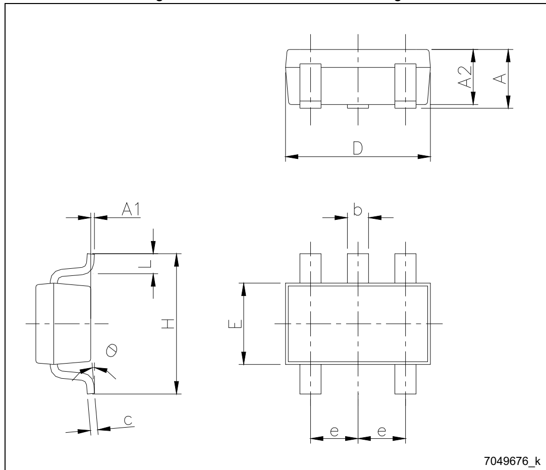
Figure 31.SOT23-5L mechanical drawings
