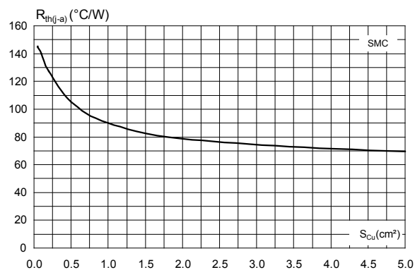
Figure 9. Thermal resistance junction to ambient versus copper surface under each lead (Epoxy printed circuit board FR4, e_{Cu} : 35 \mu m)
