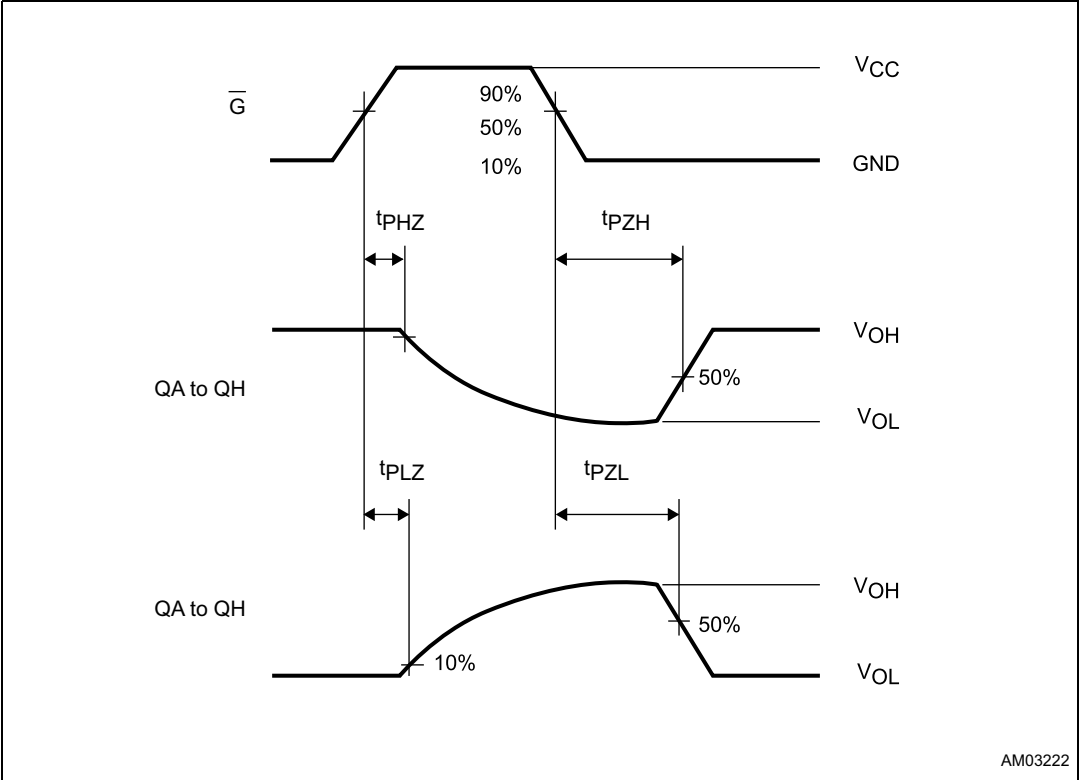
Figure 12. Waveform 6: OUTPUT ENABLE and DISABLE times ( f = 1 \text{ MHz} ; 50 % duty cycle)
