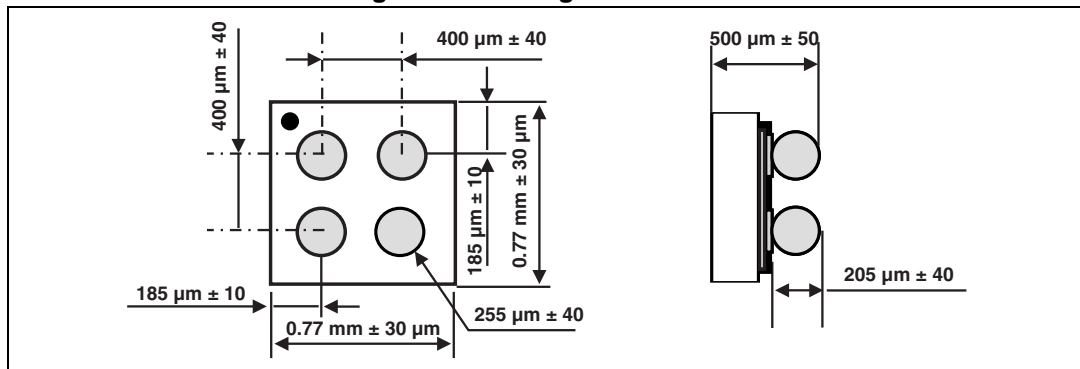
Figure 10. Package dimensions
