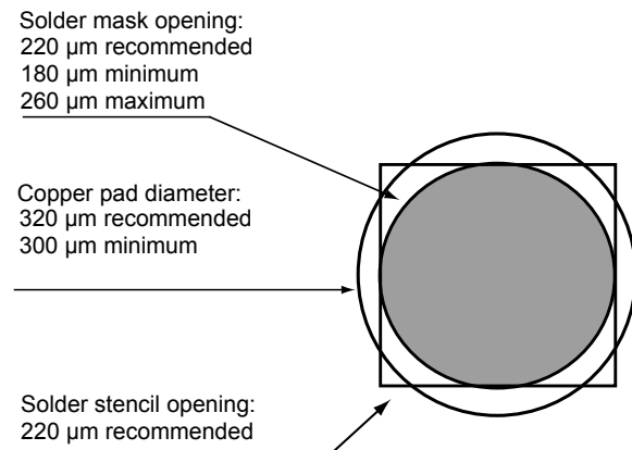
Figure 15. Footprint - 3 mils stencil - solder mask defined
