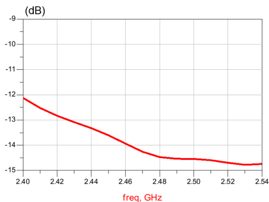
Figure 3. Return loss on SE port ( T_{\text{amb}} = 25\text{ °C} )
