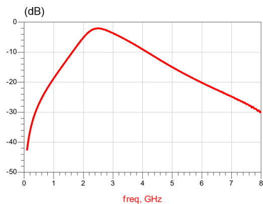
Figure 1. Transmission ( T_{\text{amb}} = 25\text{ °C} )
