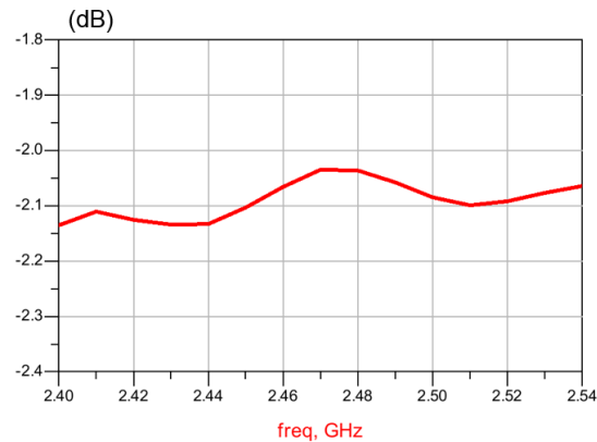
Figure 2. Insertion loss ( T_{\text{amb}} = 25\text{ °C} )
