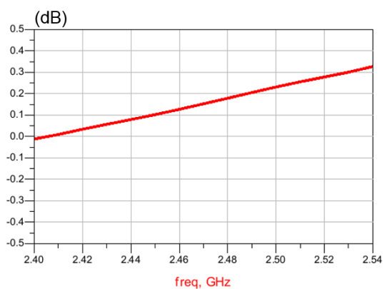
Figure 5. Amplitude imbalance ( T_{\text{amb}} = 25\text{ °C} )
