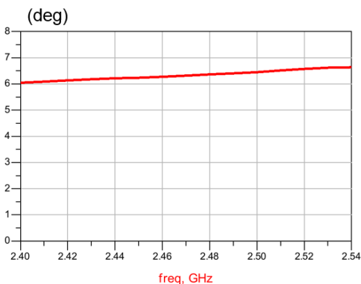
Figure 6. Phase imbalance ( T_{\text{amb}} = 25\text{ °C} )
