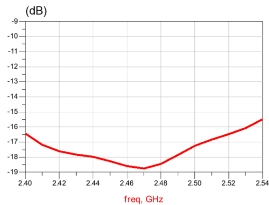
Figure 4. Return loss on DIFF port ( T_{\text{amb}} = 25\text{ °C} )
