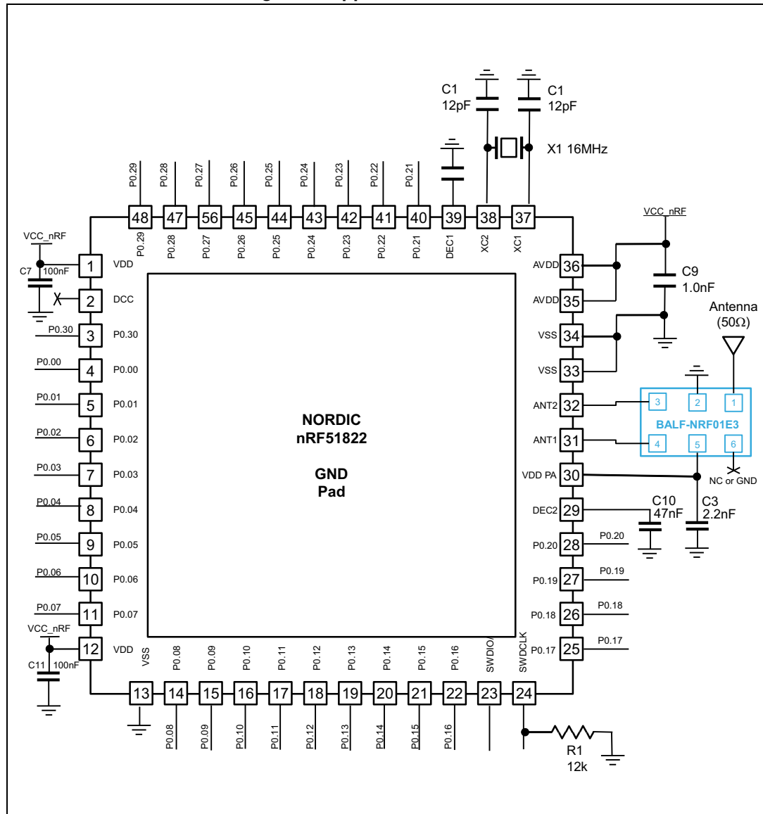
Figure 8. Application schematic
