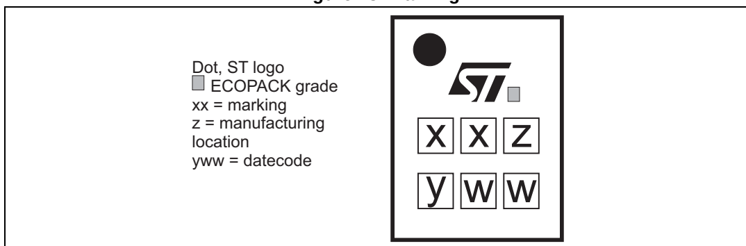
Figure 13. Marking
