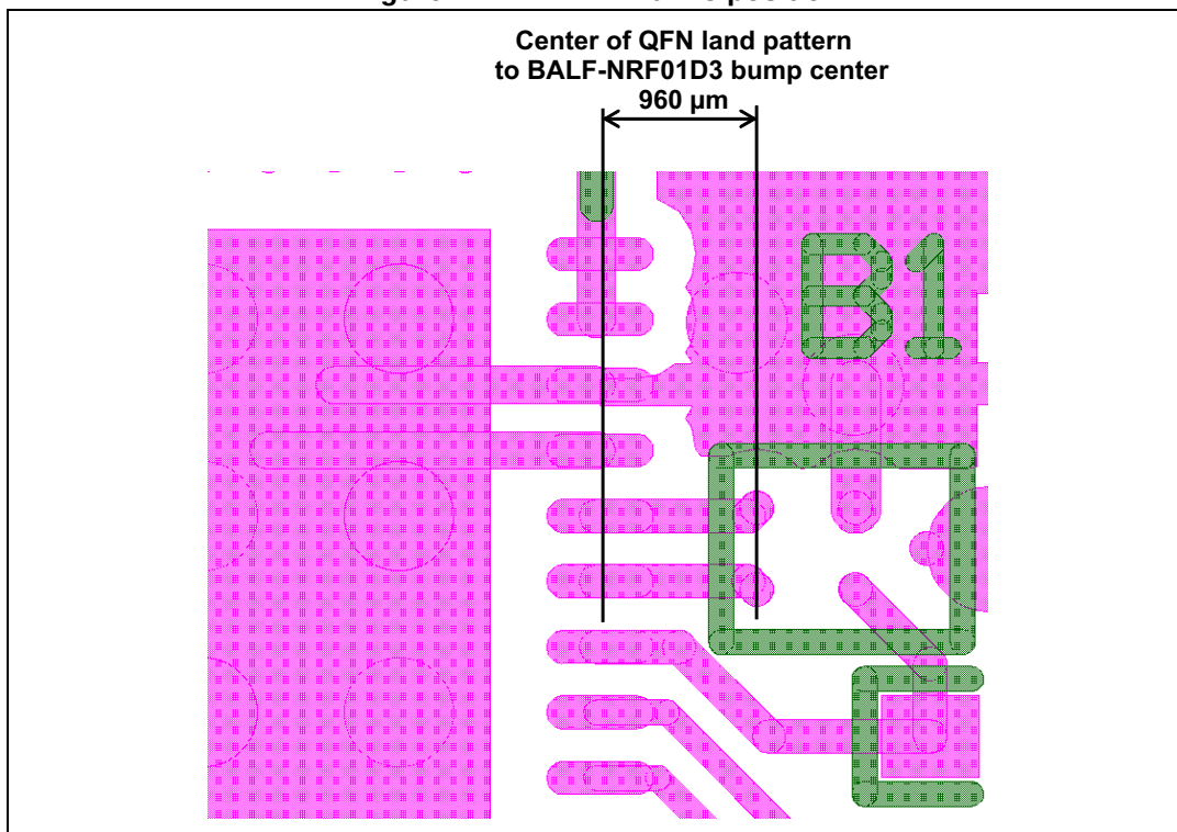
Figure 12. BALF-NRF01D3 position
