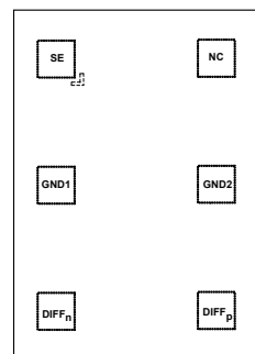
Figure 9. Top view
