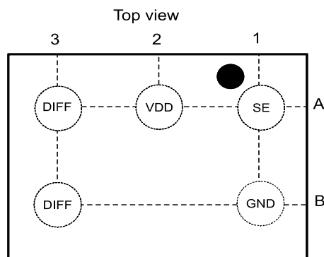
Figure 1: Pin coordinates
