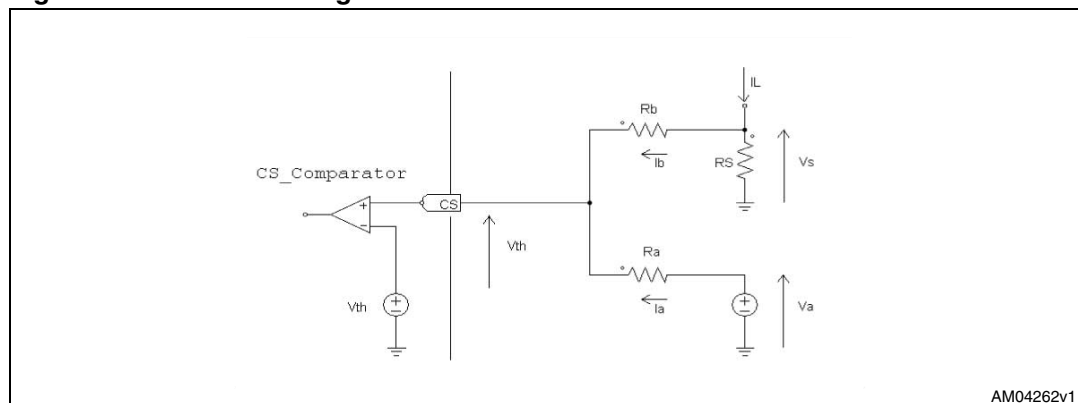
Figure 11. Current setting
