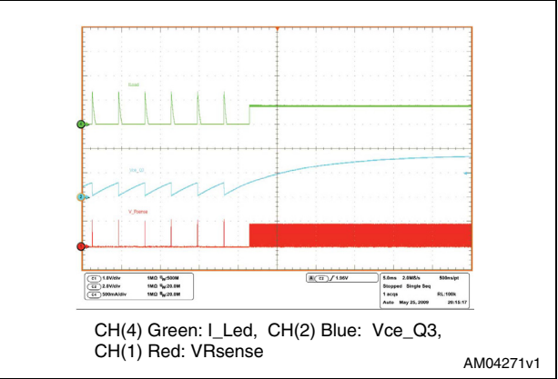
Figure 24. Short-circuit removal
