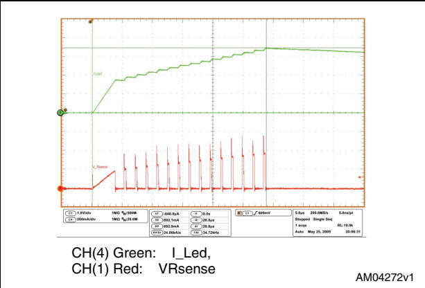
Figure 25. Short-circuit detection
