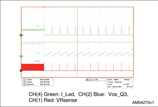
Figure 23. Short-circuit application
