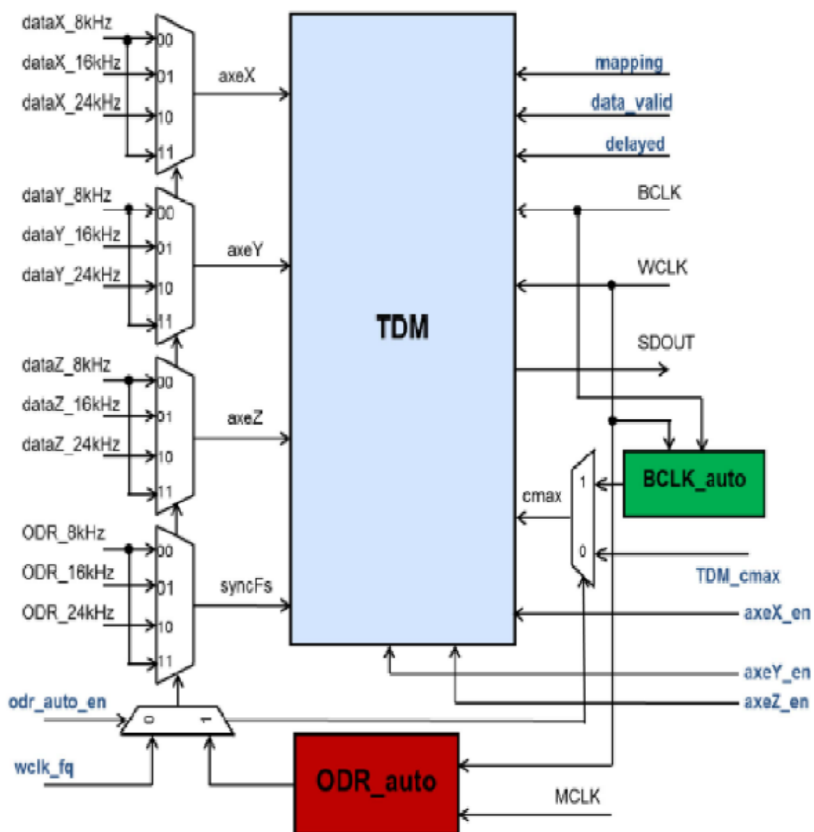
Figure 4. TDM block diagram
