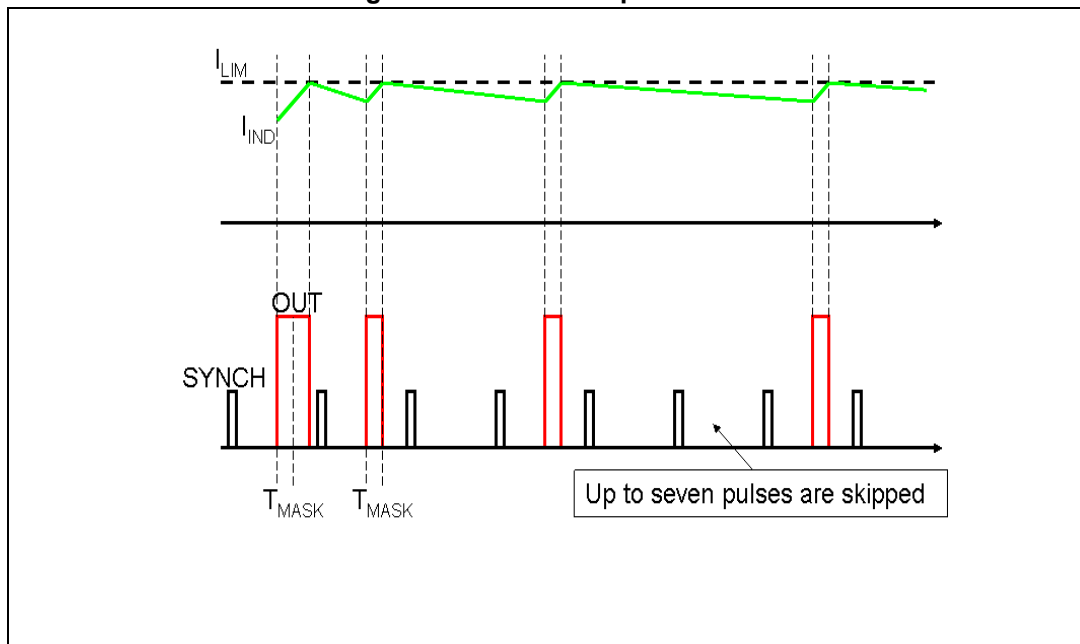
Figure 8. Overcurrent protection
