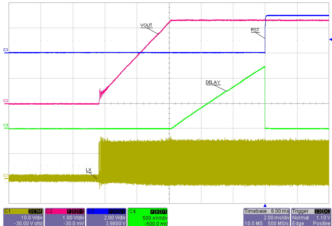
Figure 43. Voltage supervisor operation
