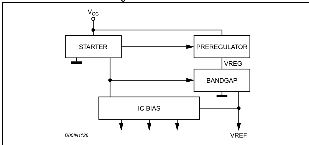
Figure 4. Internal circuit
