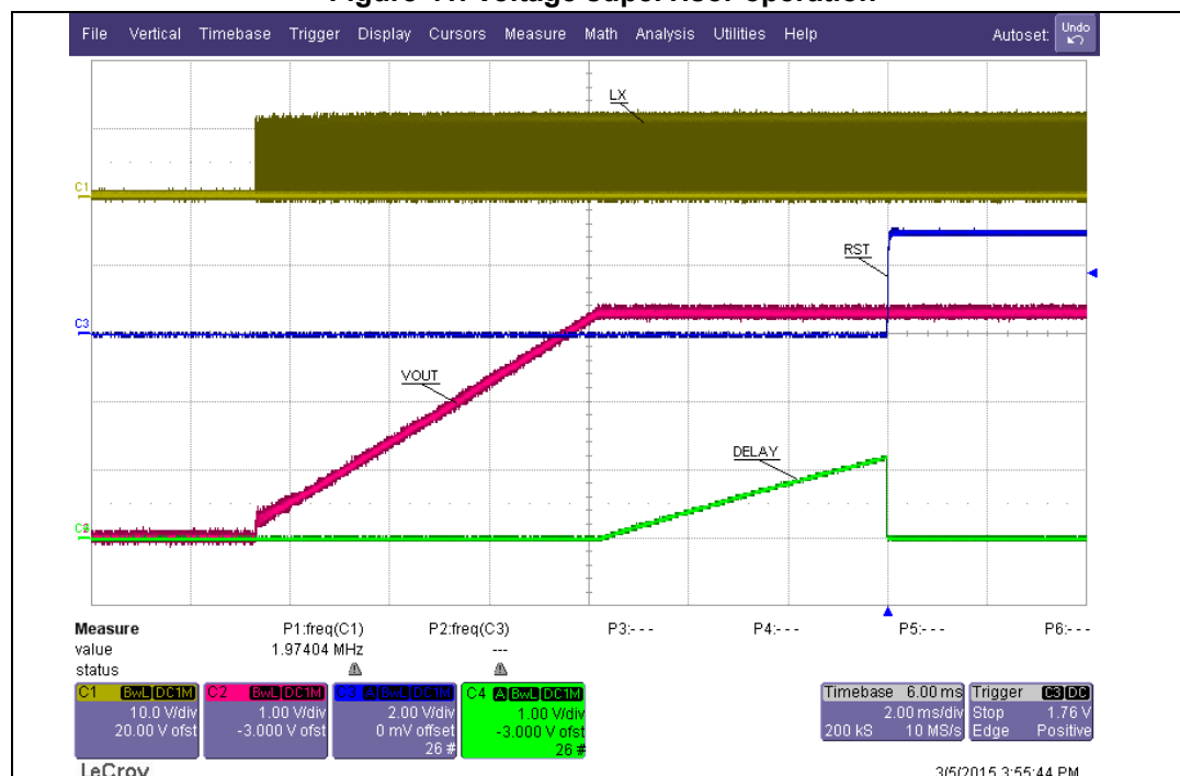
Figure 41. Voltage supervisor operation
