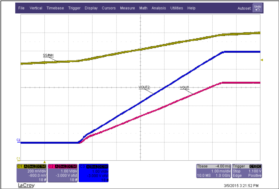
Figure 11. Ratiometric startup operation
