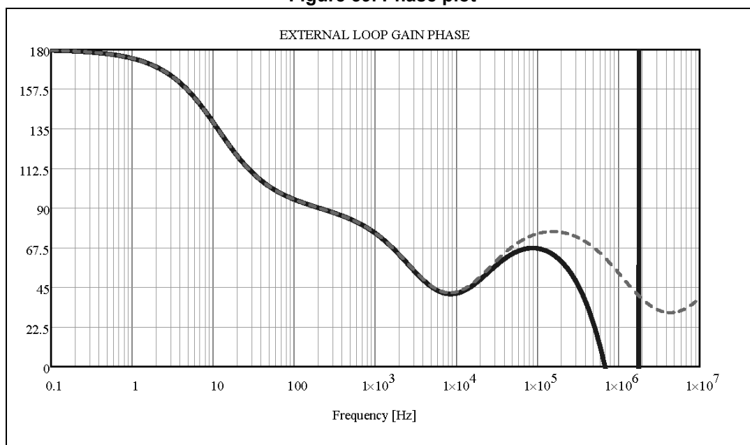
Figure 39. Phase plot
