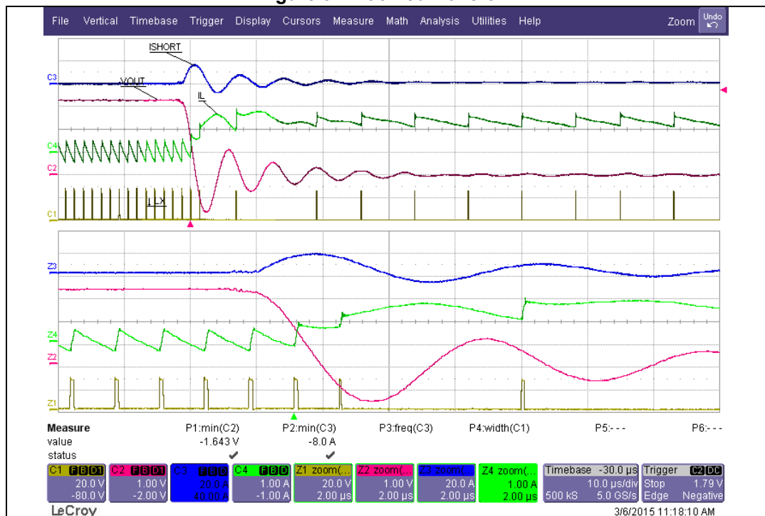
Figure 32. Zoomed waveform
