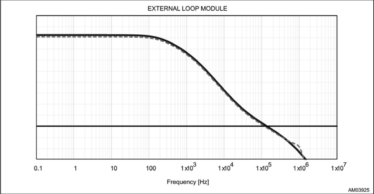
Figure 56. Magnitude Bode’s plot of A6985F (V OUT = 6 V) evaluation board
