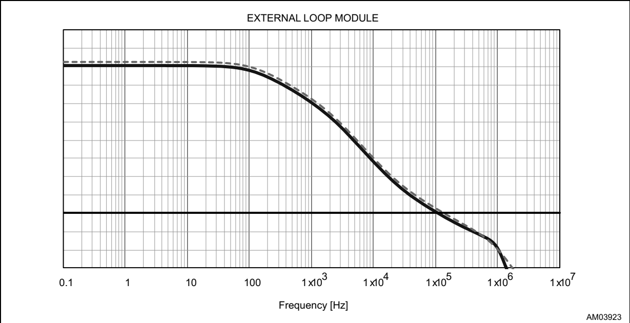
Figure 54. Magnitude Bode's plot of A6985F5V evaluation board
