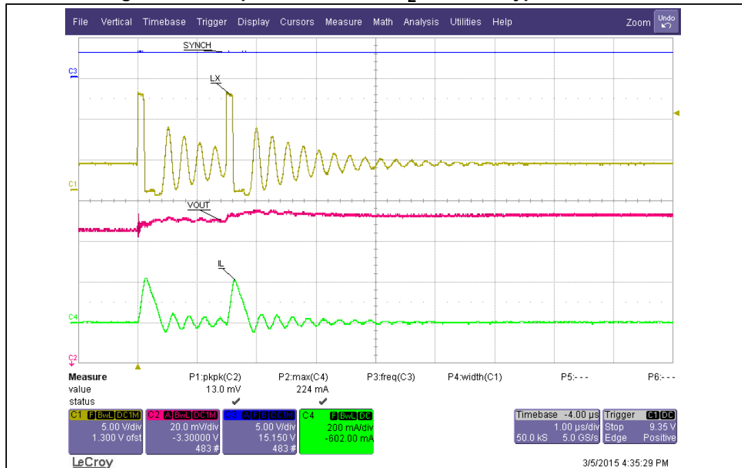
Figure 21. CM operation with IS_{SKIP_L} = 100\text{ mA typ.} at zero load
