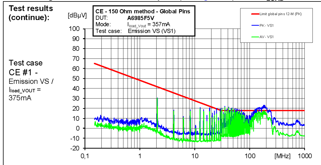
Figure 67. CE 150R at VS1 test point (see Figure 66) at 75% I_{LOAD}
