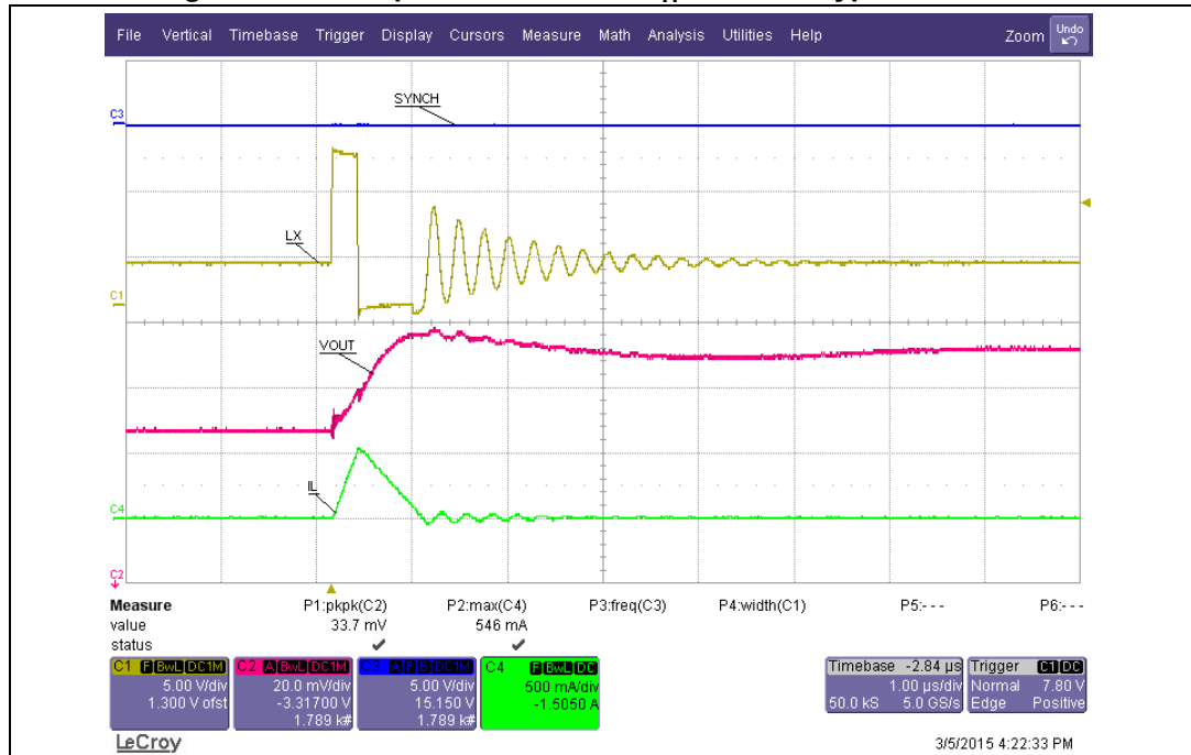
Figure 20. LCM operation with IS_{SKIP_H} = 350\text{ mA typ.} at zero load
