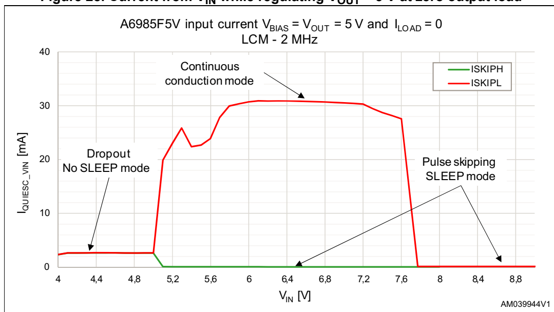
Figure 28. Current from V_{IN} while regulating V_{OUT} = 5 V at zero output load
