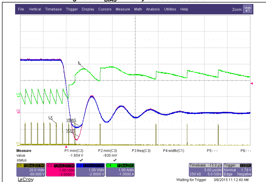
Figure 33. V_{BIAS} in heavy short-circuit event
