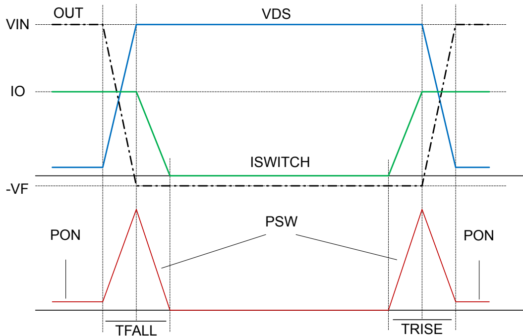
Figure 10. Switching losses
