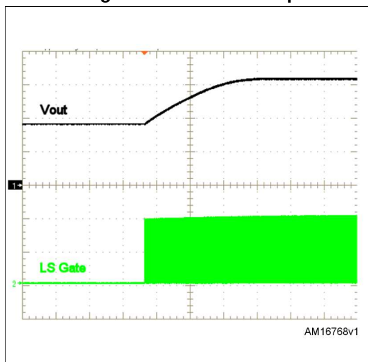
Figure 4. LS-less startup
