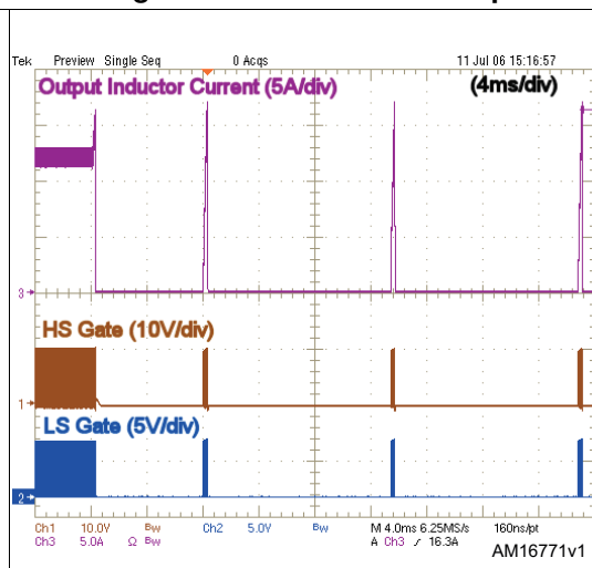
Figure 7. Overcurrent hiccup
