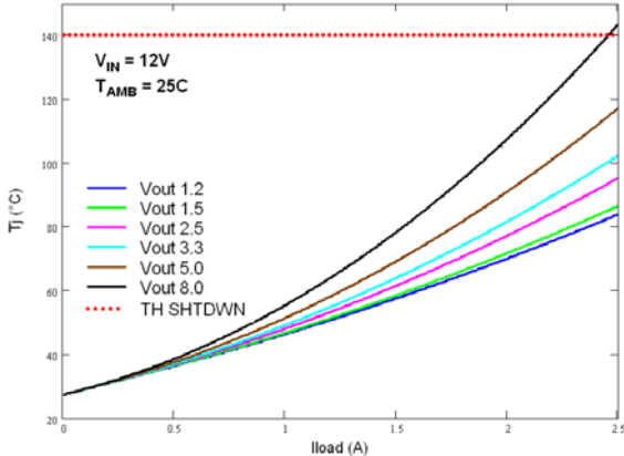
Figure 37. Junction temperature vs. output current ( V_{IN} = 12\text{V} )
