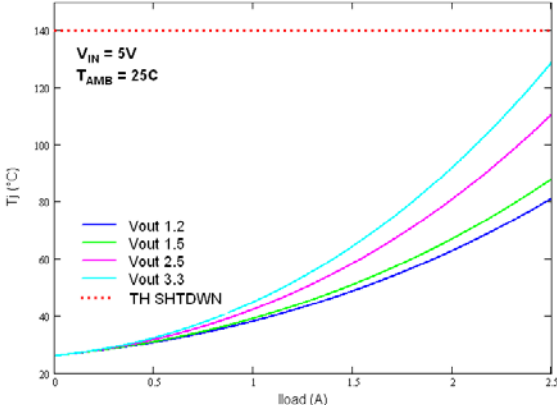
Figure 36. Junction temperature vs. output current ( V_{IN} = 5\text{V} )
