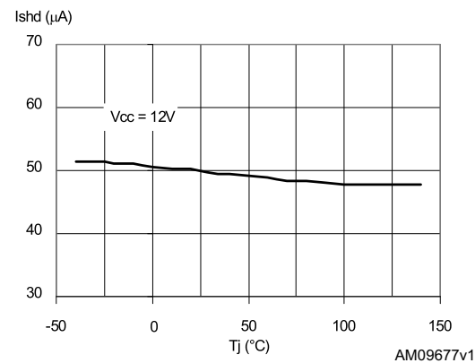
Figure 34. Shutdown current vs. junction temperature
