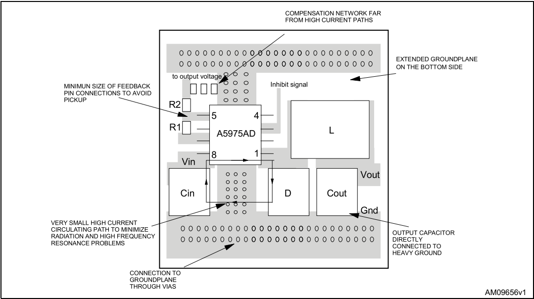
Figure 13. Layout example
