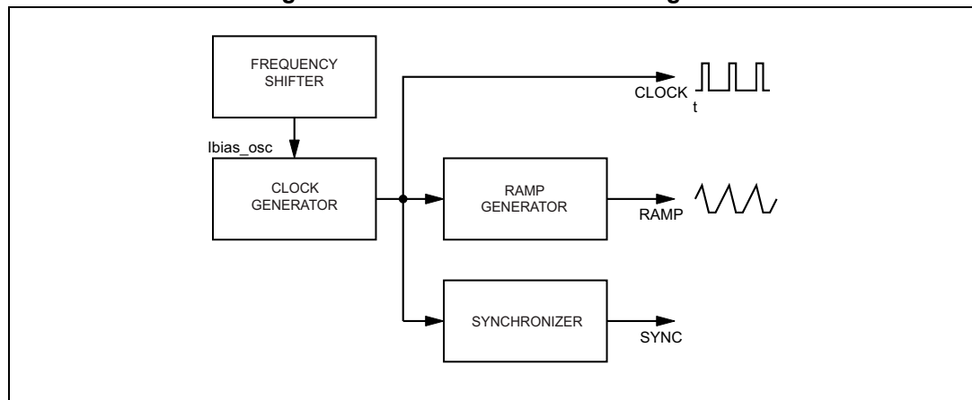
Figure 6. Synchronization example
