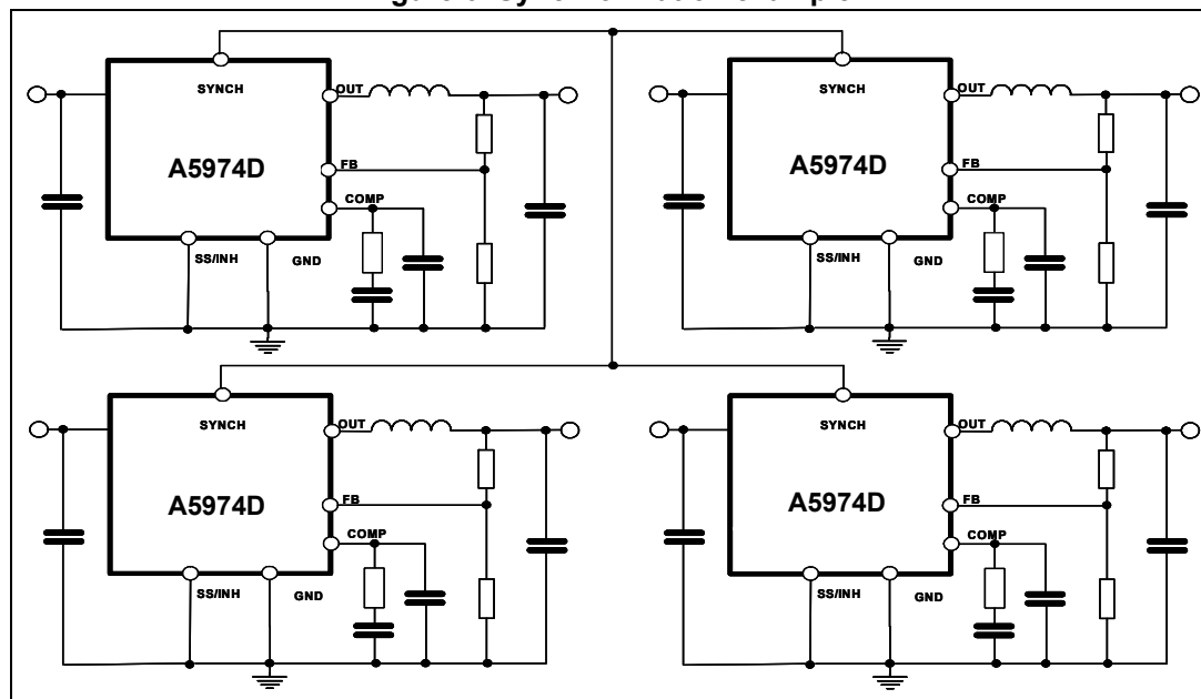
Figure 6. Synchronization example
